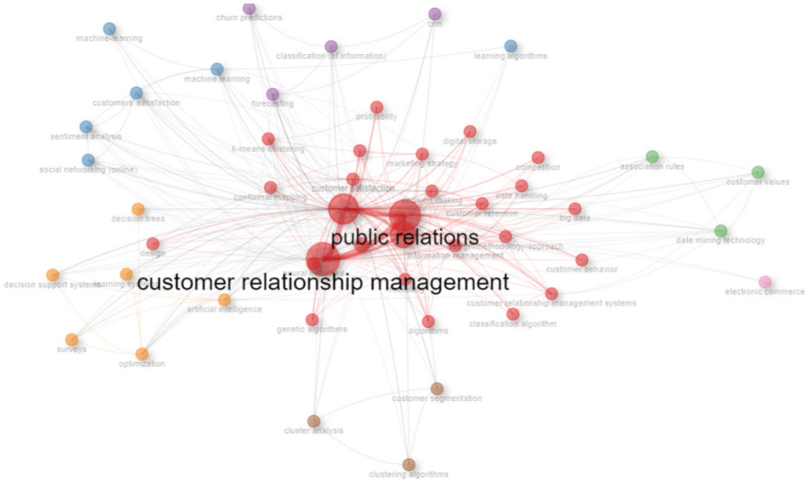
Figure 6. Co-occurrence network
