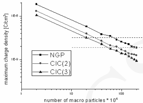
Fig. 6. Maximum deviations from the zero of charge density averaged over five middle grid layers versus the number of macro particles for three methods of charge distribution
