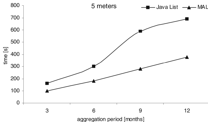
Fig. 12. Comparison of efficiency of the Java list and the MAL for 5 meters
