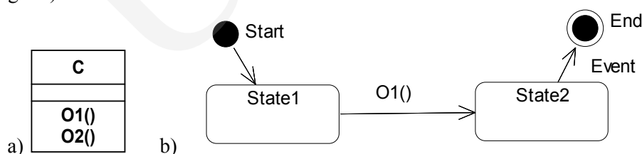
Fig. 4. a) A structural diagram – class C b) A behavioral diagram – state machine of the class C
