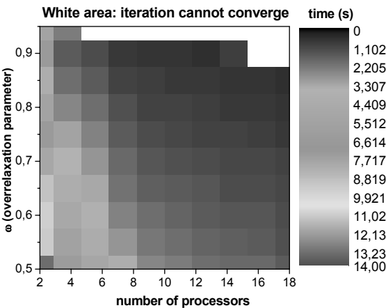
Fig. 9. A map showing the dependence of SOR computation time on the number of processors and the chosen overrelaxation parameter. If it is chosen too big, the SOR metod cannot converge
