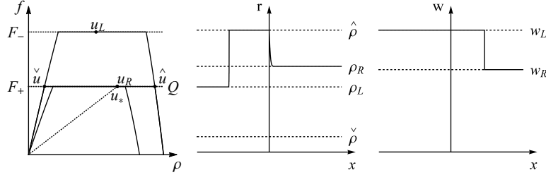
FIGURE 12. The approximate density (3.3), center, and approximate Lagrangian marker (3.4), right, corresponding to FTL model (3.2), (4.6) and the initial datum (u_L, u_R) \in \Omega^2 , left. The solution obtained by applying the Riemann solver \mathcal{RS}_{\mathfrak{R}_-, \mathfrak{R}_+} is described in (F2.e) .
