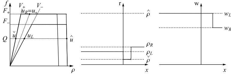
FIGURE 36. The approximate density (3.3), center, and approximate Lagrangian marker (3.4), right, corresponding to FTL model (3.2), (6.2) and initial datum (u_L, u_R) \in \Omega^2 , left. The solution obtained by applying the Riemann solver \mathcal{RS}_{\mathfrak{R}_-, \mathfrak{R}_+} is described in (FV2.e) .
