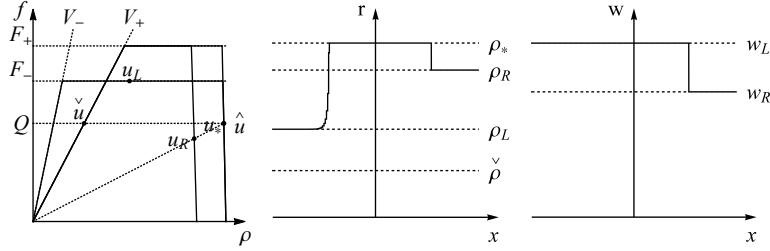
FIGURE 32. The approximate density (3.3), center, and approximate Lagrangian marker (3.4), right, corresponding to FTL model (3.2), (6.2) and initial datum (u_L, u_R) \in \Omega^2 , left. The solution obtained by applying the Riemann solver \mathcal{RS}_{\mathfrak{R}_-, \mathfrak{R}_+} is described in (FV2.a) .
