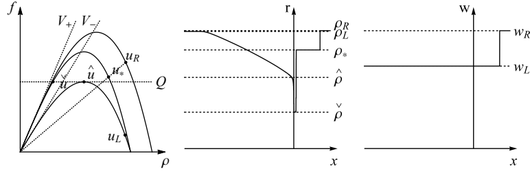
FIGURE 16. The approximate density (3.3), center, and approximate Lagrangian marker (3.4), right, corresponding to FTL model (3.2), (5.2) and the initial datum (u_L, u_R) \in \Omega^2 , left. The solution obtained by applying the Riemann solver \mathcal{RS}_{\mathfrak{R}_-, \mathfrak{R}_+} is described in (V1.c).
