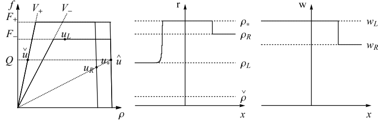
FIGURE 34. The approximate density (3.3), center, and approximate Lagrangian marker (3.4), right, corresponding to FTL model (3.2), (6.2) and initial datum (u_L, u_R) \in \Omega^2 , left. The solution obtained by applying the Riemann solver \mathcal{RS}_{\mathfrak{R}_-, \mathfrak{R}_+} is described in (FV2.c) .
