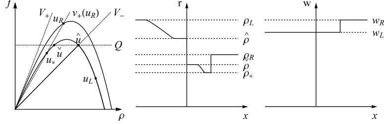
FIGURE 21. The approximate density (3.3), center, and approximate Lagrangian marker (3.4), right, corresponding to FTL model (3.2), (5.3) and initial datum (u_L, u_R) \in \Omega^2 , left. The solution obtained by applying the Riemann solver \mathcal{RS}_{\mathfrak{R}_-, \mathfrak{R}_+} is described in (V2.b) .
