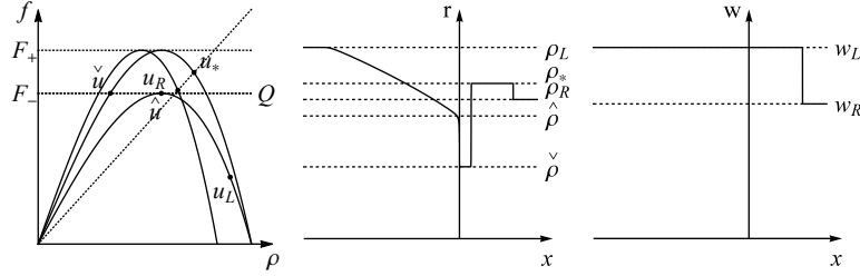
FIGURE 6. The approximate density (3.3), center, and approximate Lagrangian marker (3.4), right, corresponding to FTL model (3.2), (4.4) and the initial datum (u_L, u_R) \in \Omega^2 , left. The solution obtained by applying the Riemann solver \mathcal{RS}_{\mathfrak{R}_-, \mathfrak{R}_+} is described in (F1.e) .
