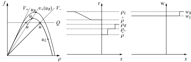
FIGURE 22. The approximate density (3.3), center, and approximate Lagrangian marker (3.4), right, corresponding to FTL model (3.2), (5.3) and initial datum (u_L, u_R) \in \Omega^2 , left. The solution obtained by applying the Riemann solver \mathcal{RS}_{\mathfrak{R}_-, \mathfrak{R}_+} is described in (V2.c) .
