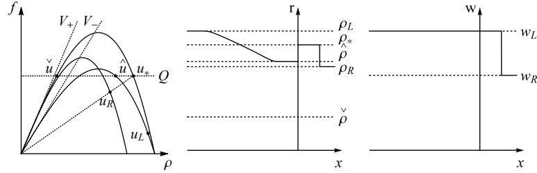
FIGURE 18. The approximate density (3.3), center, and approximate Lagrangian marker (3.4), right, corresponding to FTL model (3.2), (5.2) and the initial datum (u_L, u_R) \in \Omega^2 , left. The solution obtained by applying the Riemann solver \mathcal{RS}_{\mathfrak{R}_-, \mathfrak{R}_+} is described in (V1.e).
