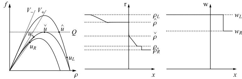
FIGURE 15. The approximate density (3.3), center, and approximate Lagrangian marker (3.4), right, corresponding to FTL model (3.2), (5.2) and the initial datum (u_L, u_R) \in \Omega^2 , left. The solution obtained by applying the Riemann solver \mathcal{RS}_{\mathfrak{R}_-, \mathfrak{R}_+} is described in (V1.b).
