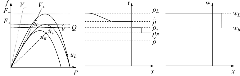
FIGURE 26. The approximate density (3.3), center, and approximate Lagrangian marker (3.4), right, corresponding to FTL model (3.2), (6.1) and initial datum (u_L, u_R) \in \Omega^2 , left. The solution obtained by applying the Riemann solver \mathcal{RS}_{\mathfrak{R}_-, \mathfrak{R}_+} is described in (FV1.a) .
